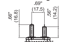
A Two 10-32 studs: .66"(AUX); .56"(BAT)
