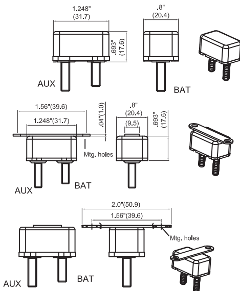
Circuit Breaker w/ METAL Cover
