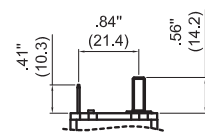
E One .25" Q.C.(AUX); One 10-32 stud(BAT)
